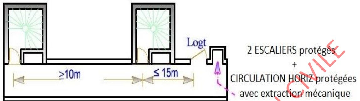
Figure 25 : Solution n°1.
